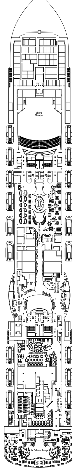
DECK 7 MYKONOS
