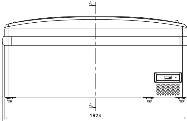
TectoFreeze IS2 Freez 183-FC-CE °C -23 to -18 or -1 to +5
