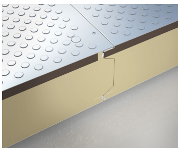
Hygienic floor underlap
