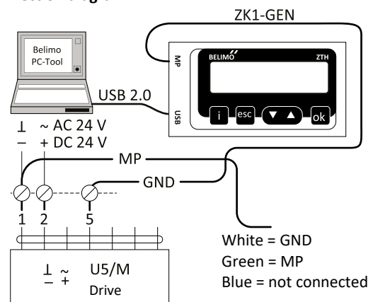
Connection diagram 2
