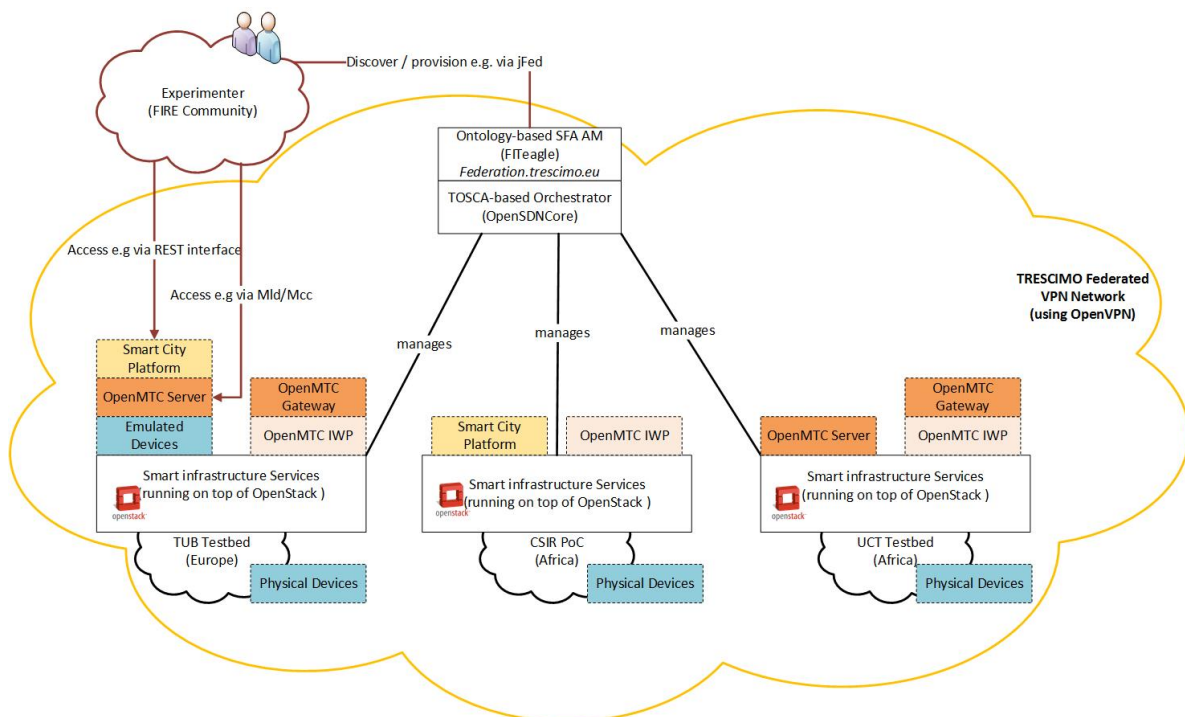
Figure 2: Functional Architecture of Federated TRESIMO Testbed
